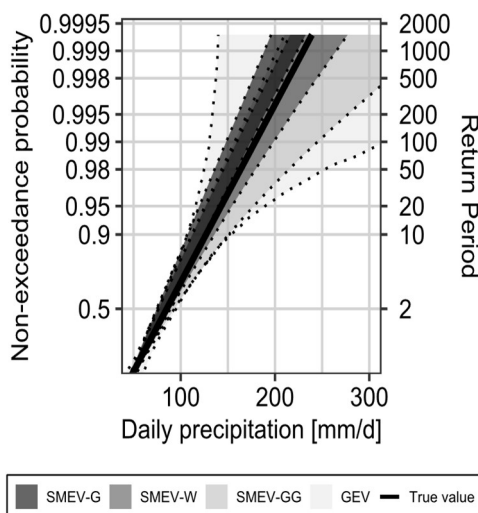
図3 模擬発生データに基づいた補正值の分布 Distributions of annual maximum daily rainfall corrected in simulated data.
